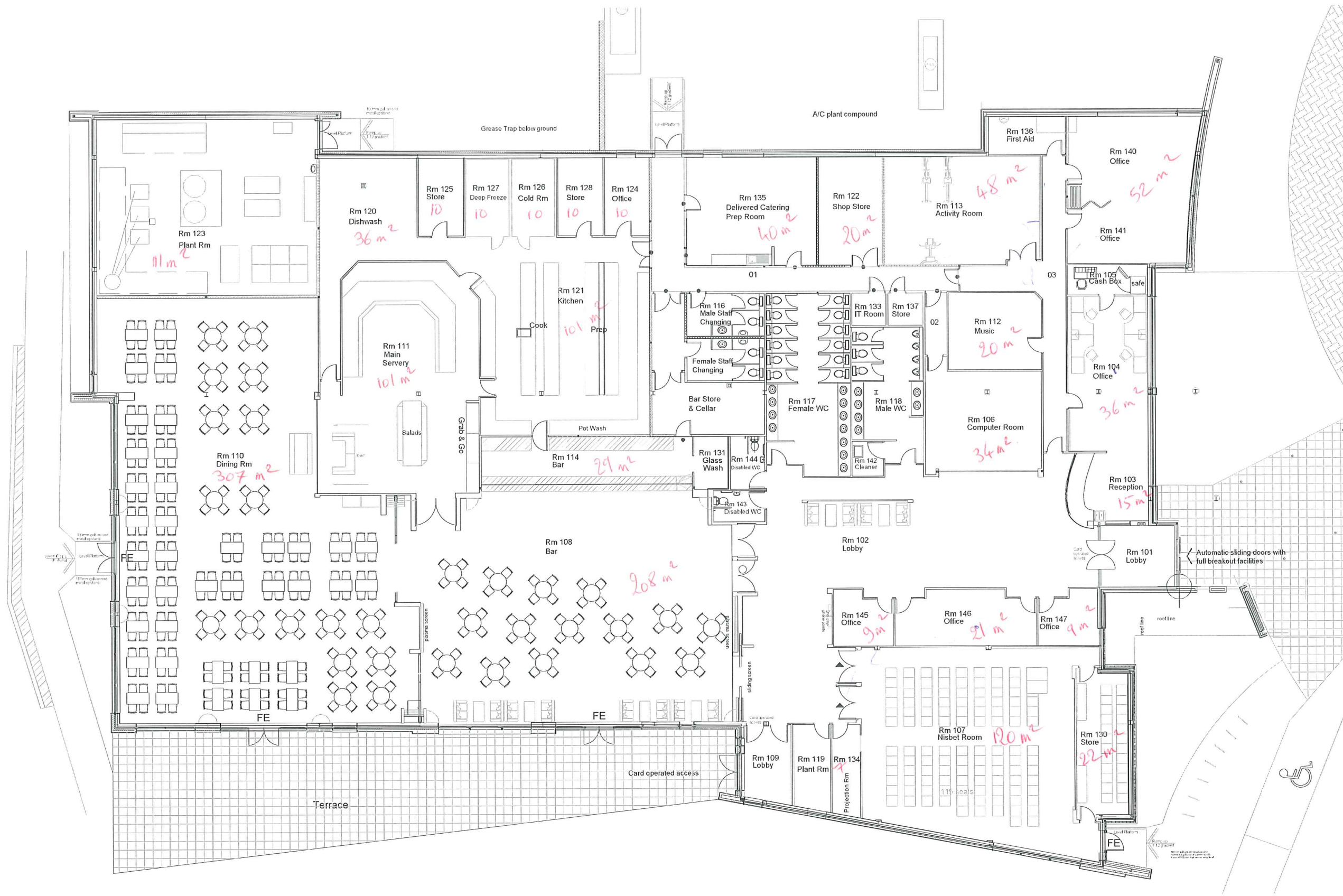
FLOOR PLAN DAVID RUSSELL APARTMENTS FACILITIES BLOCK
